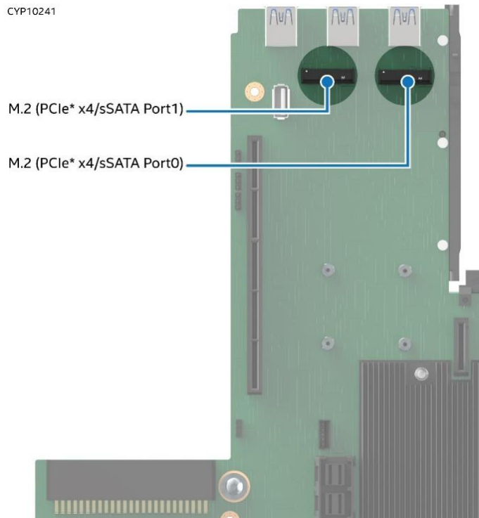
Figure 90. M.2 Module Connector Location
