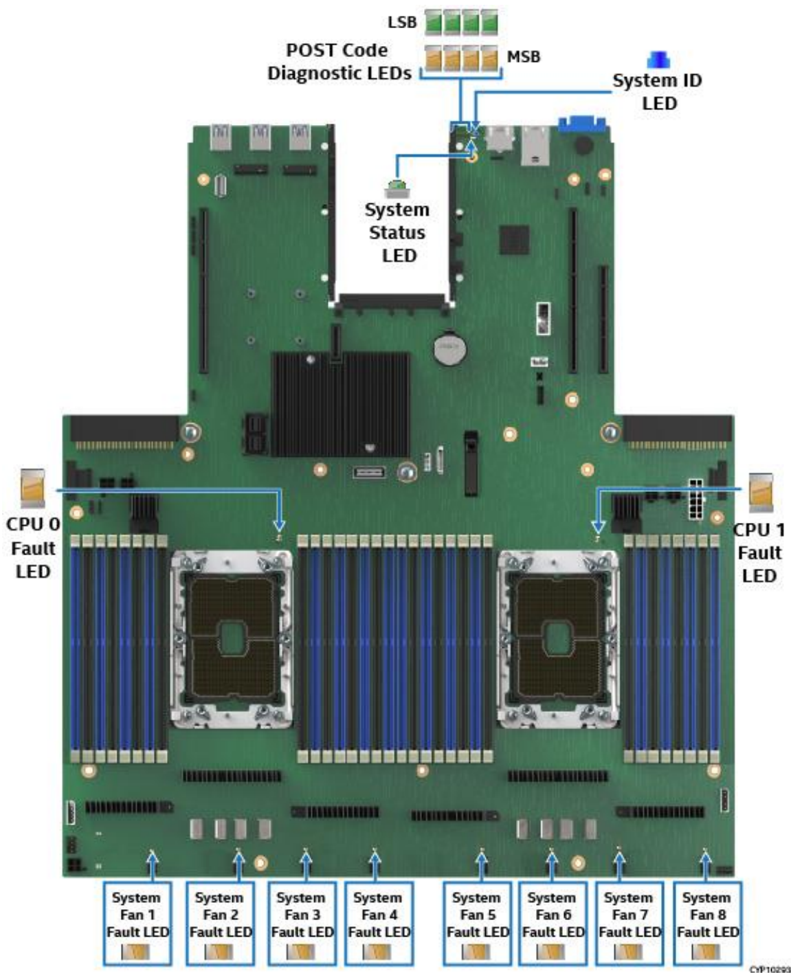
Figure 101. Intel® Server System M50CYP1UR Family Onboard LEDs
