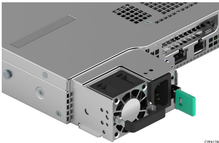
Figure 32. Power Supply Module Partially Out of Chassis
