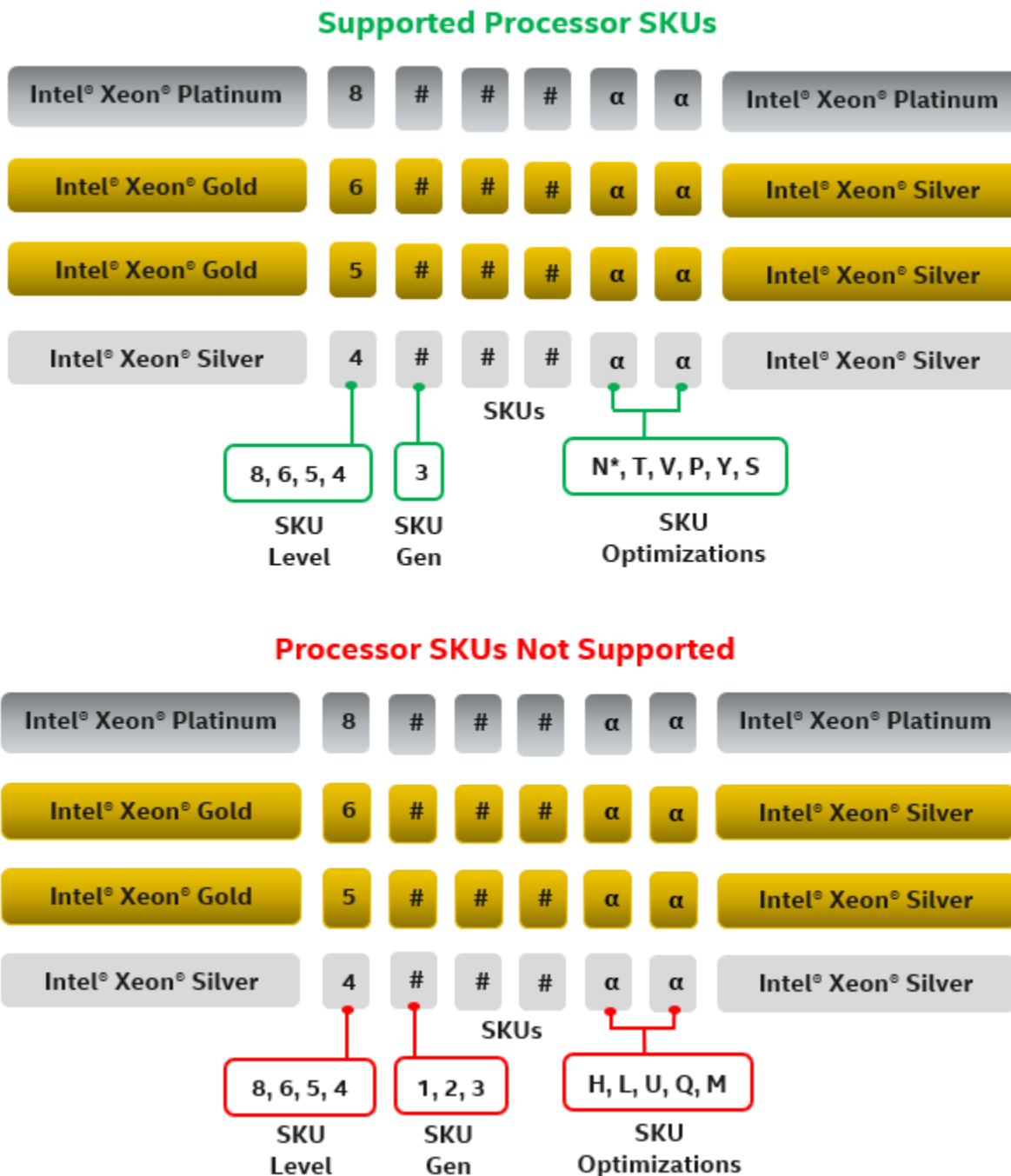
Figure 23. 3 rd Gen Intel® Xeon® Scalable Processor Identification
