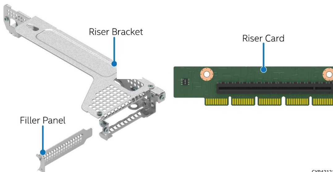
Figure 43. Riser Bracket Components
