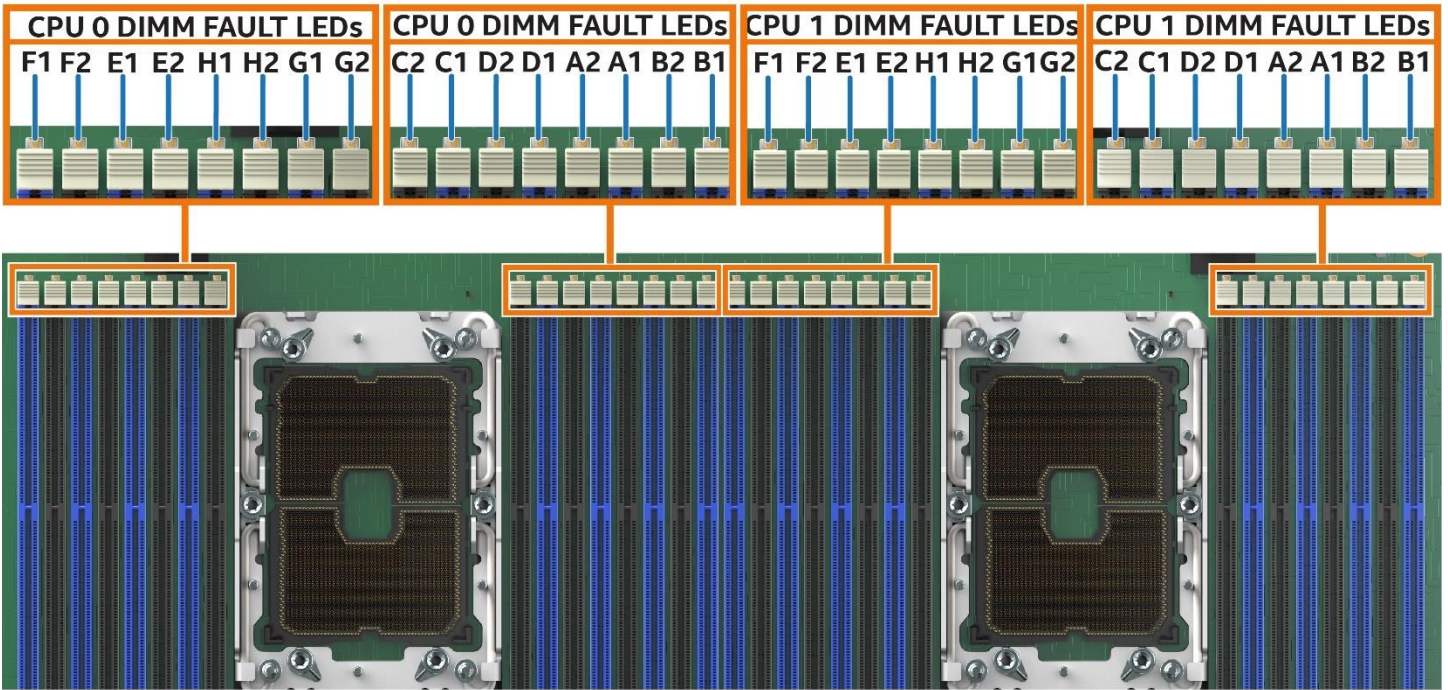
Figure 10. Intel® Light-Guided Diagnostics – DIMM Fault LEDs
