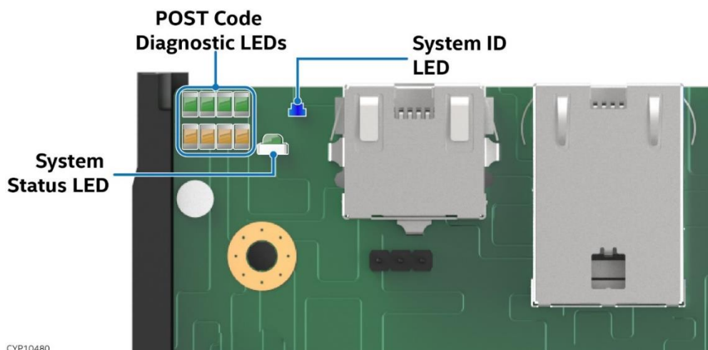
Figure 102. Exploded View of POST Code Diagnostic, System ID, and System Status LEDs
