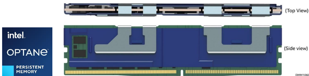
Figure 26. Intel® Optane™ Persistent Memory 200 Series Module
