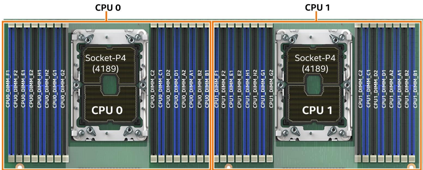
Figure 29. Intel® Server System M50CYP1UR Family Memory Slot Layout
