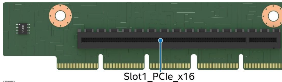
Figure 49. PCIe* Riser Card for Riser Slot #1
