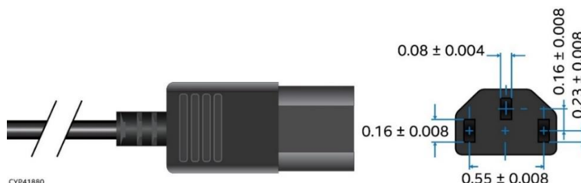
Figure 35. AC Power Cord Specification
