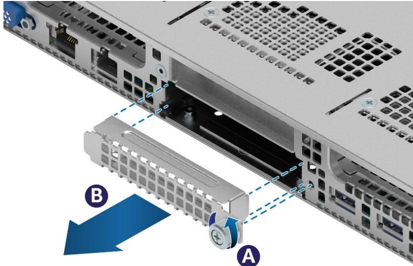
Figure 55. OCP* Adapter Bay Filler Removal
