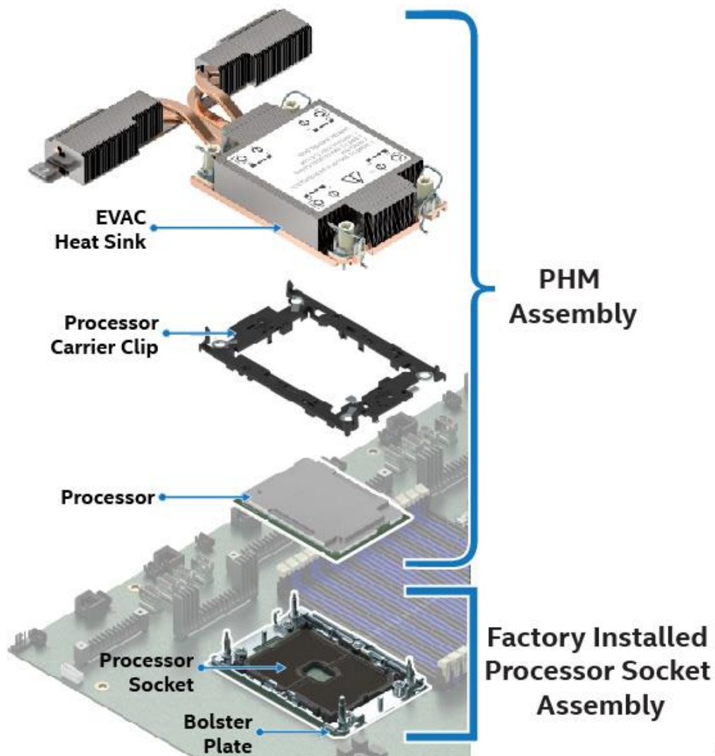
Figure 22. PHM Components and Processor Socket Reference Diagram
