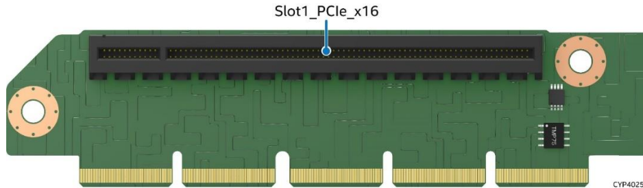
Figure 50. PCIe* Riser Card for Riser Slot #2
